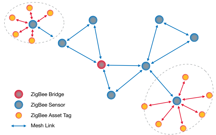
Mesh network routing permits path formation from any source device to any destination device.
